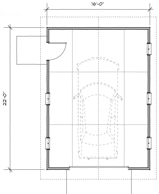
FLOOR PLAN
